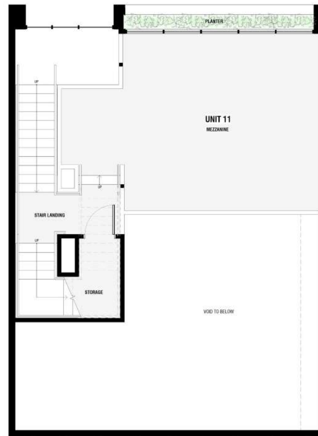
UNIT 11 - MEZZANINE FLOOR PLAN
