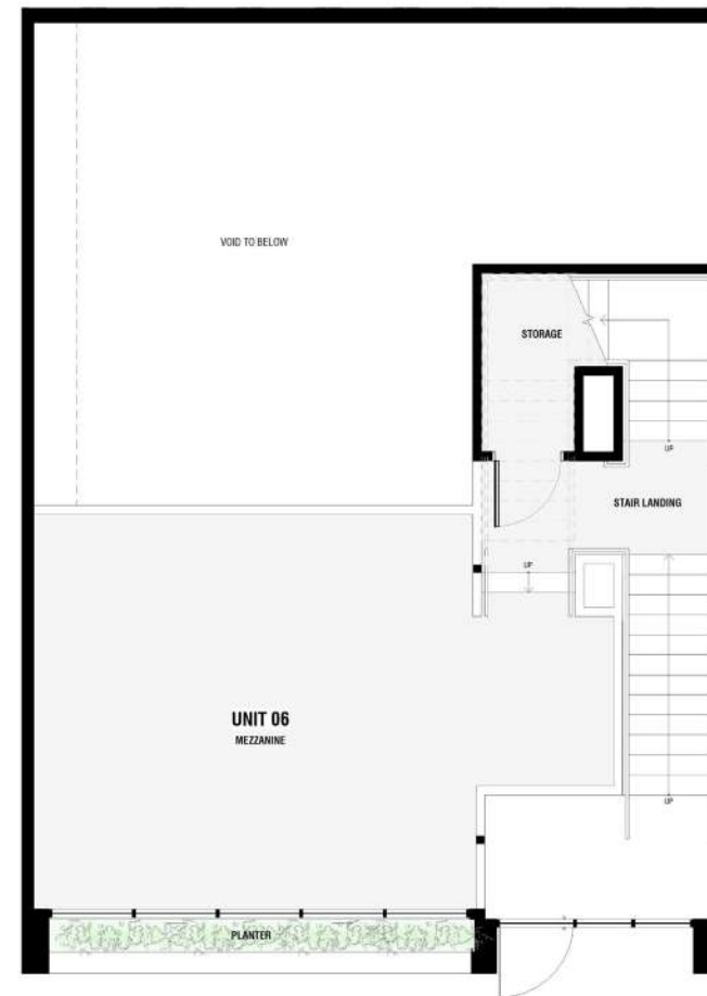
UNIT 6 - MEZZANINE FLOOR PLAN
