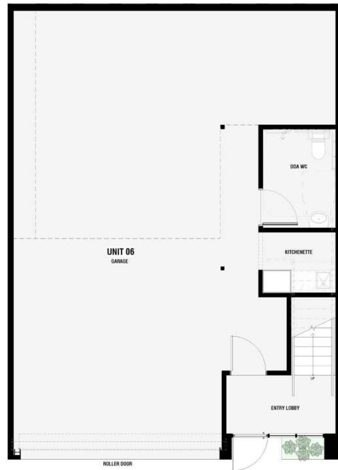
UNIT 6 - GROUND FLOOR PLAN
