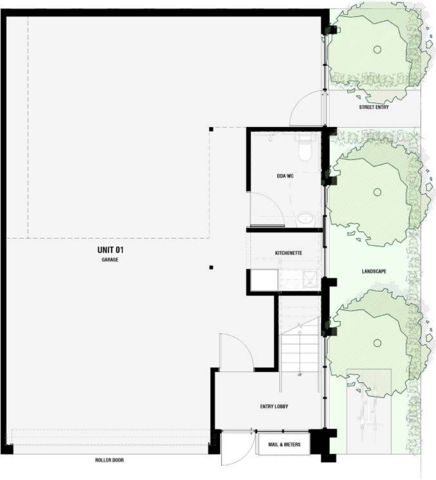
UNIT 2 - GROUND FLOOR PLAN
