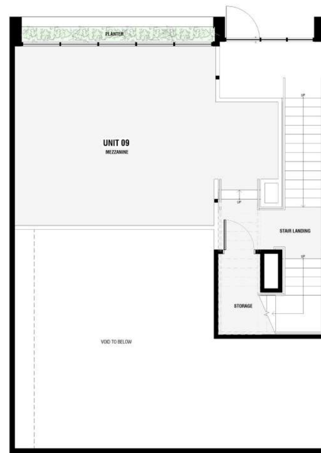
UNIT 9 - MEZZANINE FLOOR PLAN
