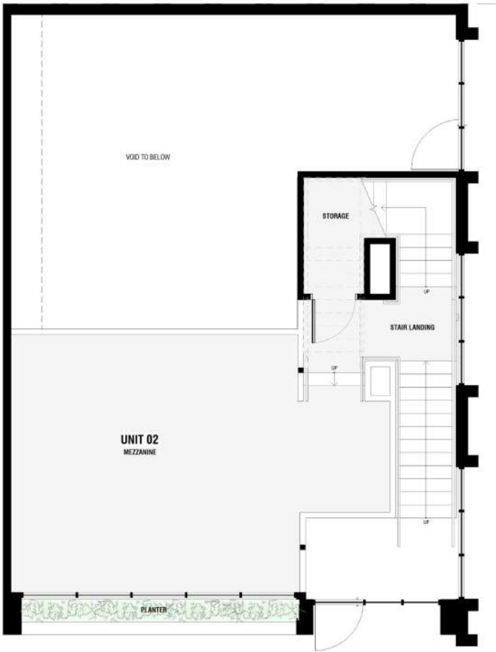
UNIT 2 - MEZZANINE FLOOR PLAN
