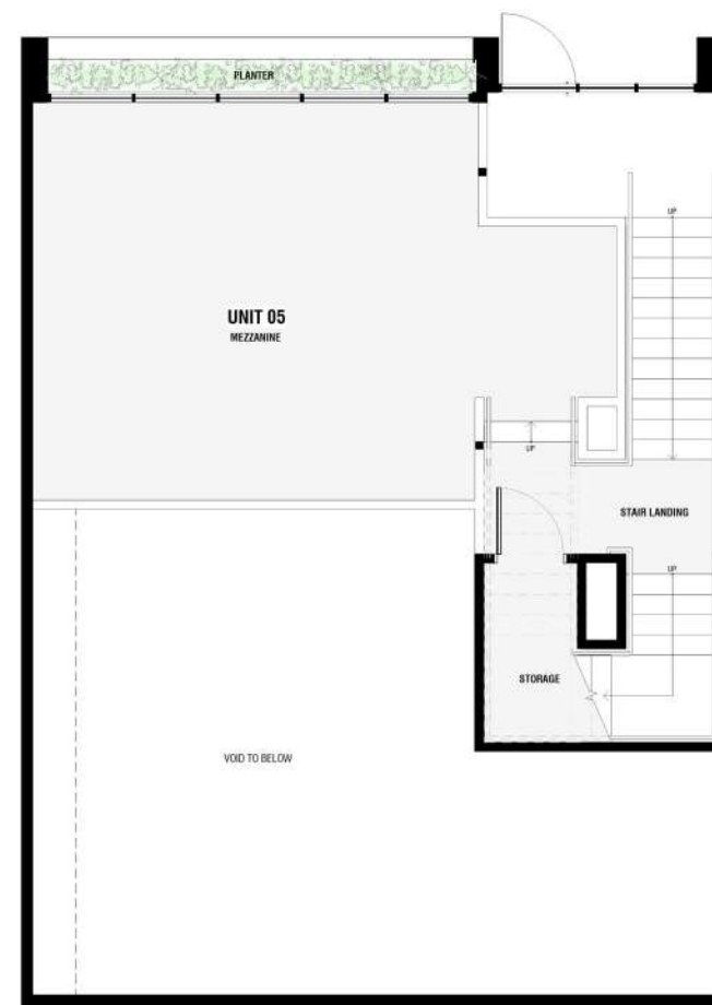
UNIT 5 - MEZZANINE FLOOR PLAN
